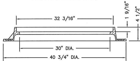
COVER SECTION
