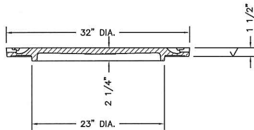
COVER SECTION
